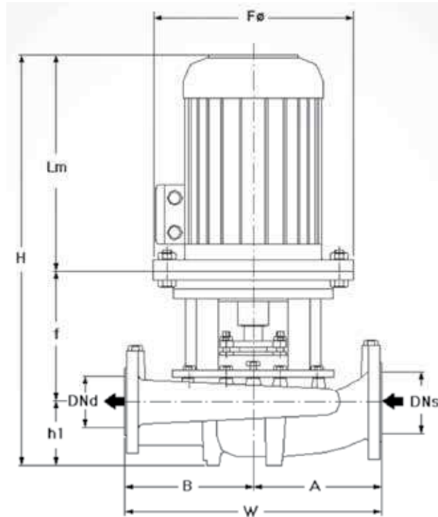
YPH Series Fire Pumps Dimension Table
