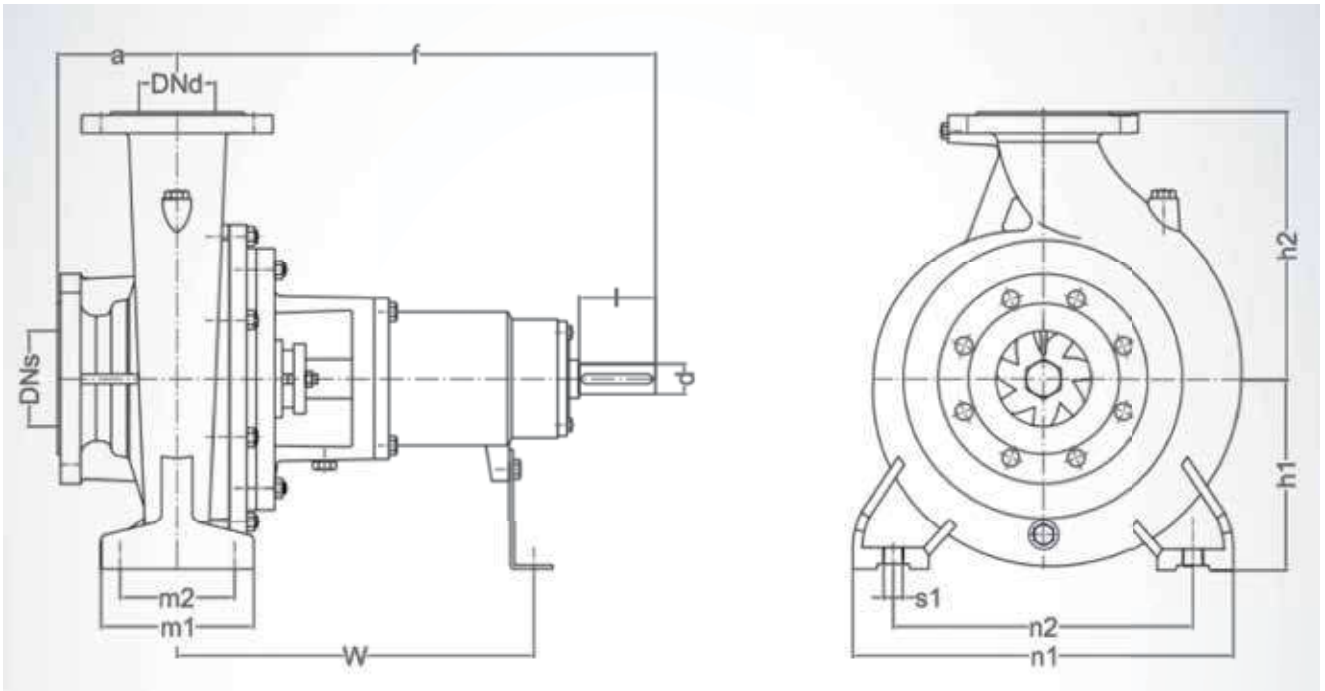
General Pump Sizes
